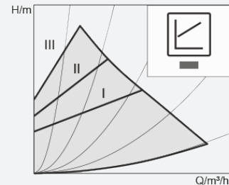
Variable differential pressure \Delta p-v (I, II, III)
