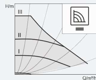
Constant speed (I, II, III)
