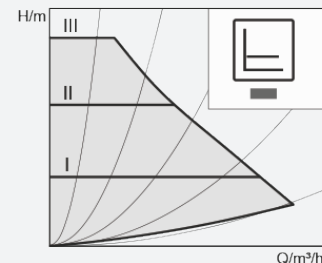
Constant differential pressure \Delta p-c (I, II, III)
