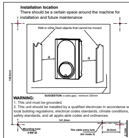
1 x Installation template
